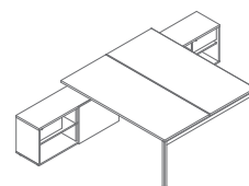
BOYL41 1800-1902 / 3210 / 740 188.1 kg
